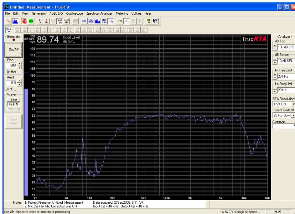
200Hz cross over – as above
