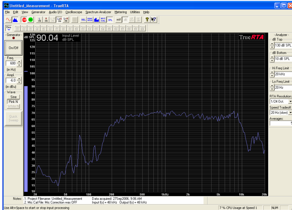
160 Hz cross over – mic at horn mouth – pink noise
